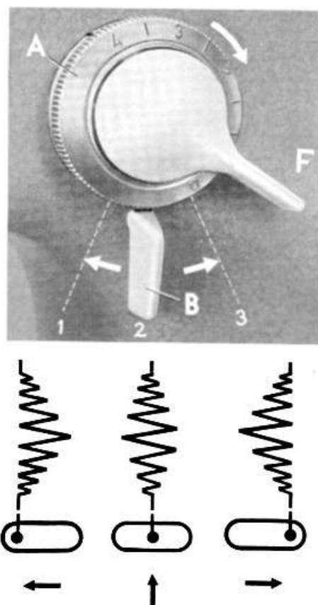
Fig. 39 Lever B changes the position of the needle in the needle plate slot
