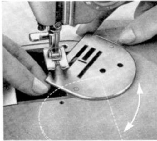
Figs. 36 & 37 Changing the needle plate
