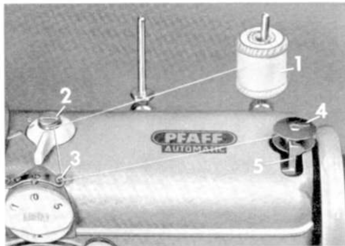
Fig. 31 Bobbin winding
