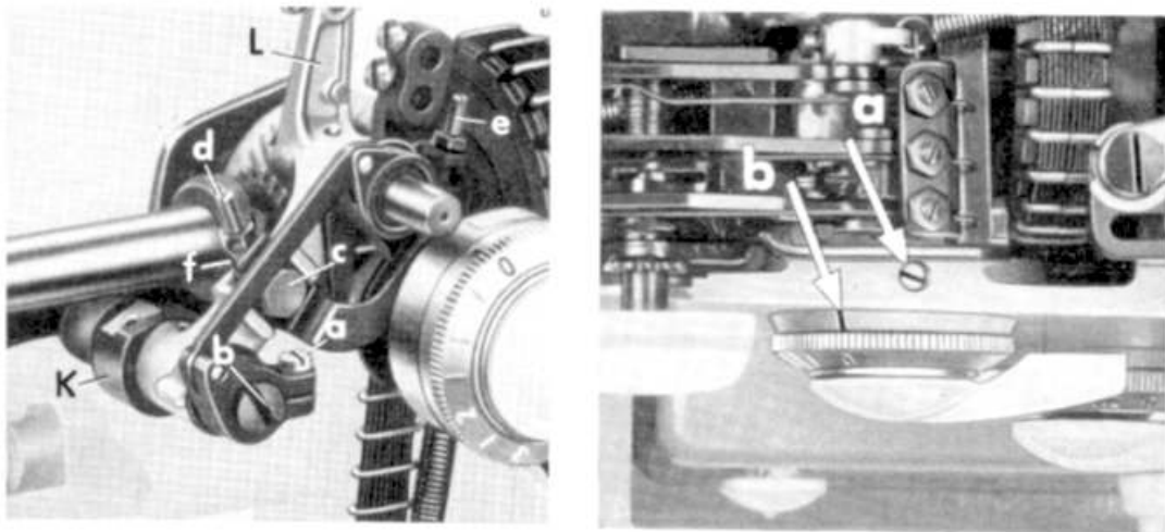
Figs. 104 & 105 Zeroing and centering the needle
