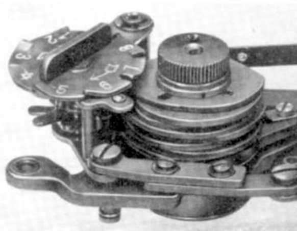
Fig. 97 The heart of the Automatic – the cam assembly
