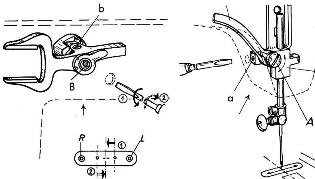
Figs. 106 & 107 Centering the needle in the needle plate slot (in both drawings the machine is pictured as seen from the rear)
