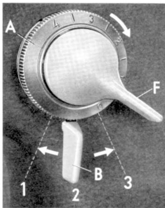
Fig. 101 Stitch width control of the Pfaff 260 (360) (present model)
